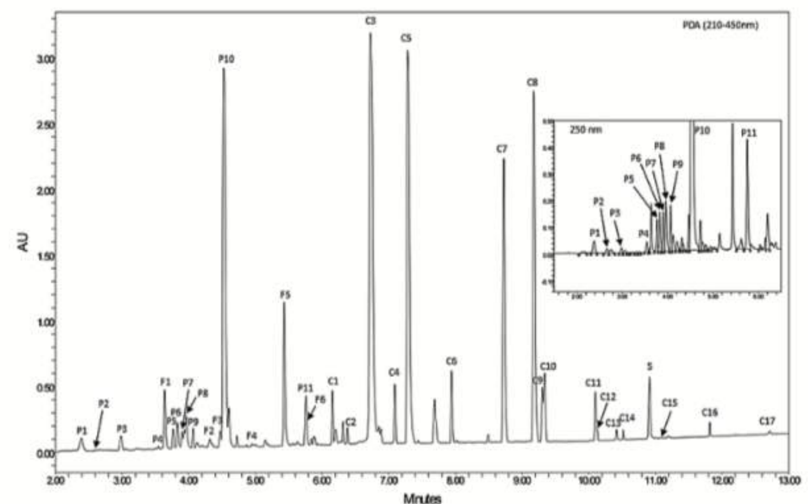
Signature saffron™ characterization by U-HPLC.
